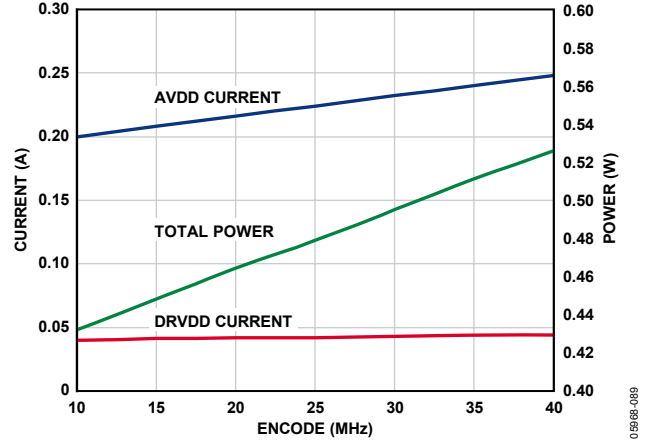
Figure 57. Supply Current vs. f_{SAMPLE} for f_{IN} = 10.3 MHz, AD9212-40
