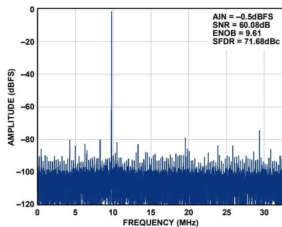
Figure 20. Single-Tone 32k FFT with f_{IN} = 120 MHz, AD9212-65
