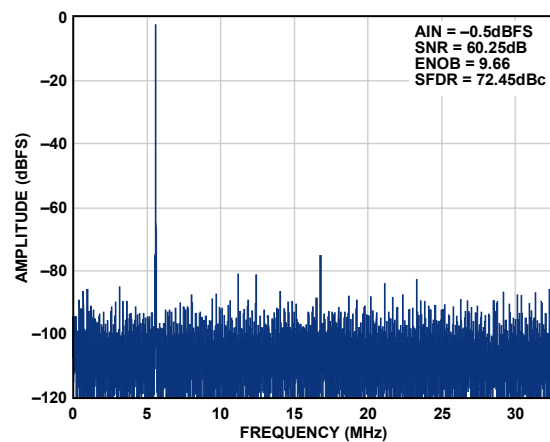
Figure 19. Single-Tone 32k FFT with f_{IN} = 70 MHz, AD9212-65
