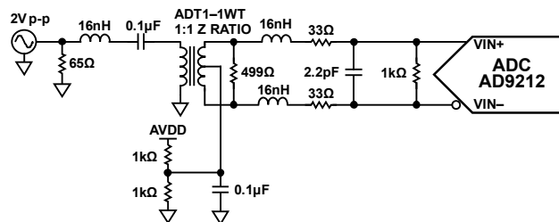
Figure 48. Differential Transformer-Coupled Configuration for IF Applications
