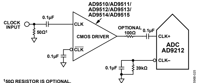
Figure 54. Single-Ended 1.8 V CMOS Sample Clock
