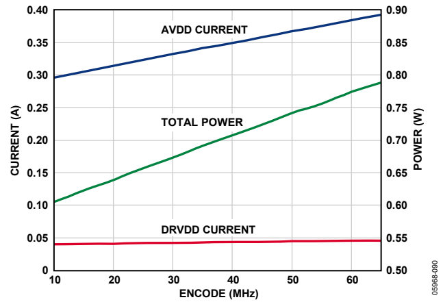
Figure 58. Supply Current vs. f_{SAMPLE} for f_{IN} = 10.3 MHz, AD9212-65
